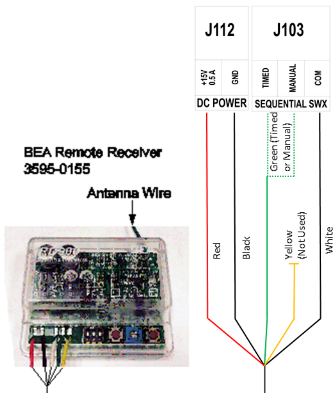
Figure 36: BEA Receiver
